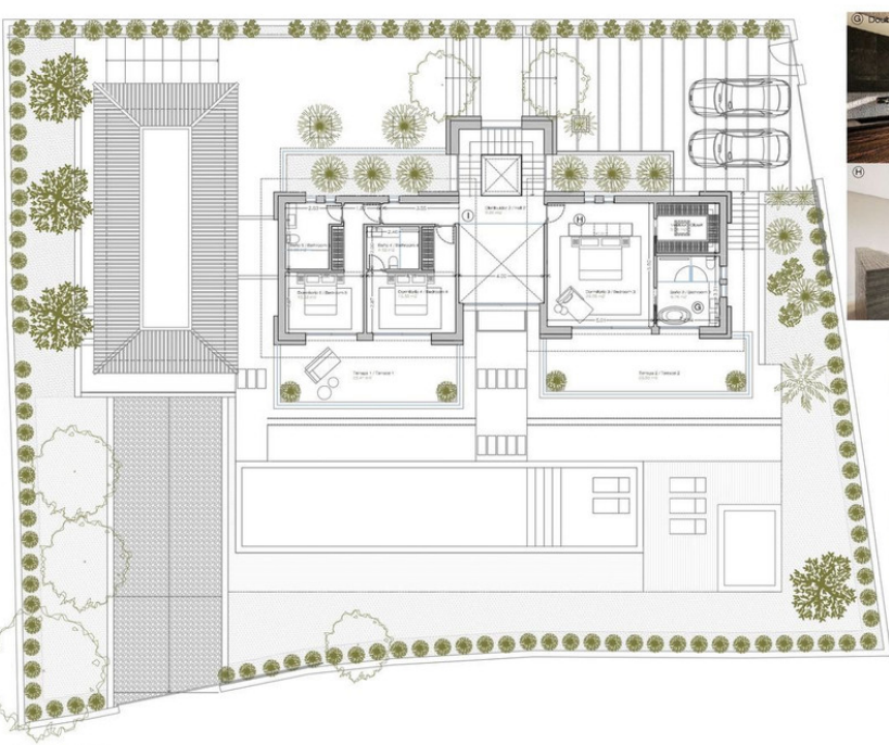
PLANTA ALTA / FIRST FLOOR 102.61 m 2 (102.61)
