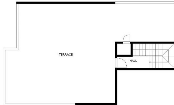
FLOOR 2
