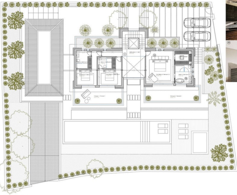
PLANTA ALTA / FIRST FLOOR 126.61 m 2
