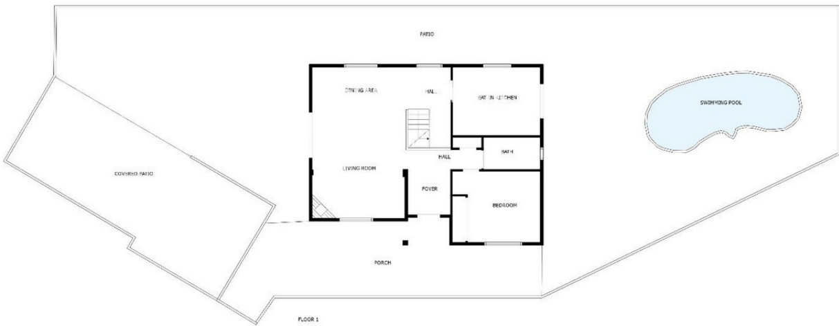
FLOOR 1
