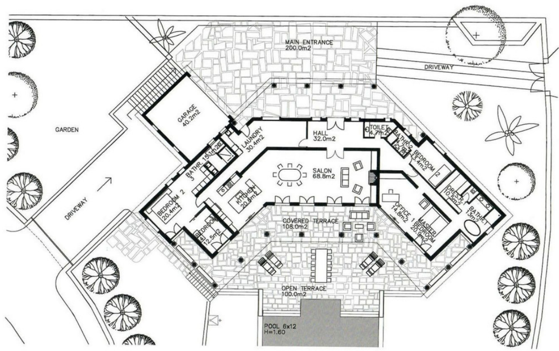
GROUND FLOOR 0 2 4 6 8 10 m
