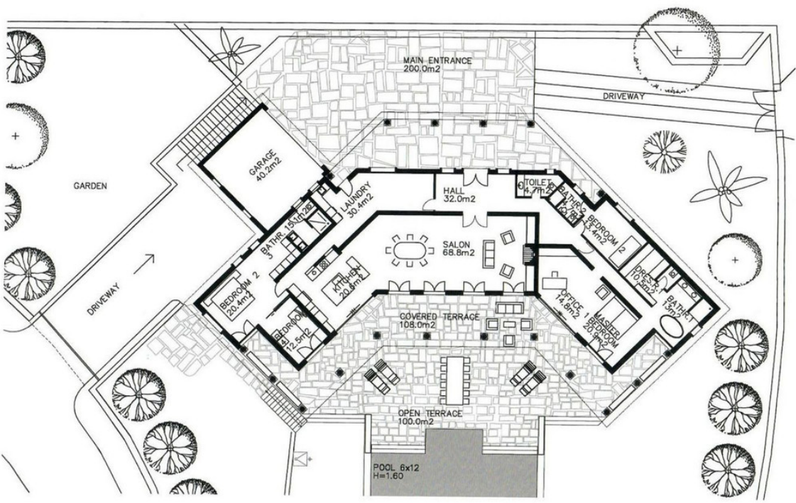
GROUND FLOOR 0 2 4 6 8 10 m
