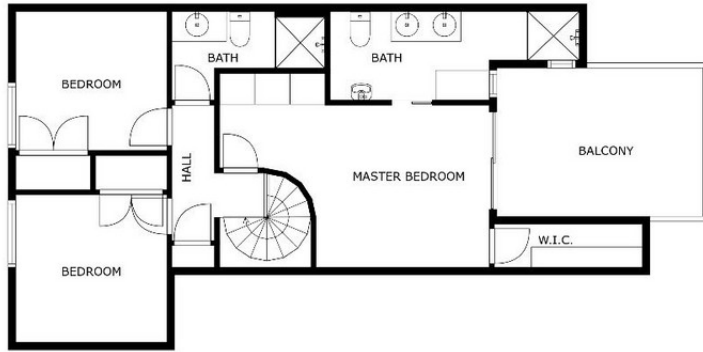
FLOOR 2
